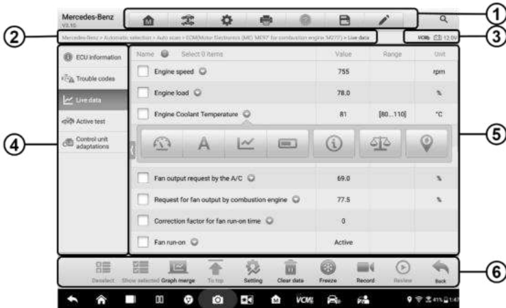
Figure 4-18 Sample Live Data Screen
