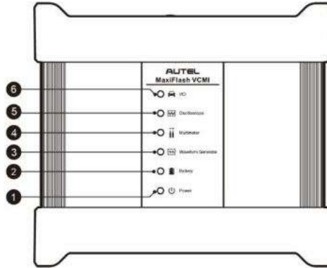
VCM Front View
