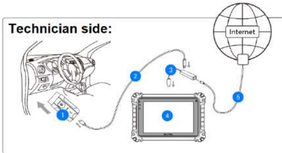
Figure 8-1 Sample connection diagram on Technician side
