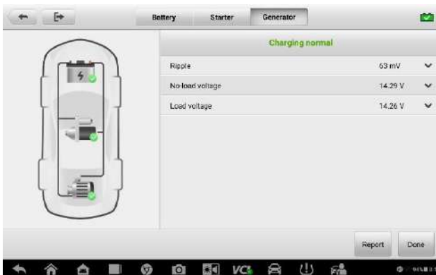
Figure 9-12 Sample Generator Test Result Screen
