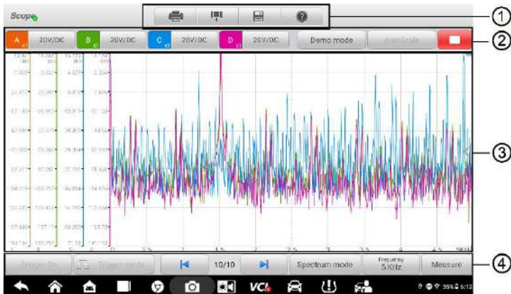
Figure 19-4 Sample Oscilloscope Application Screen Layout
