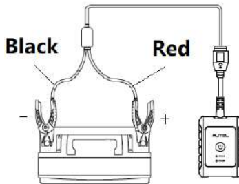
Figure 9-2 Connecting to a Battery
