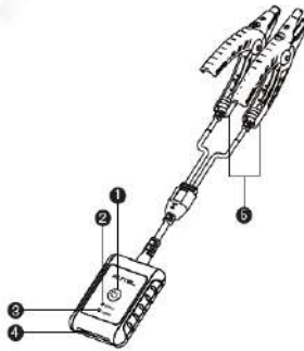
Figure 9-1 MaxiBAS BT506 Tester
